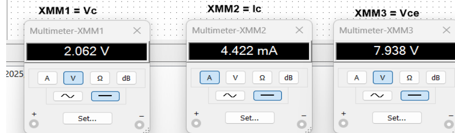
Fig : Fixed Bias Circuit (BD-135)
