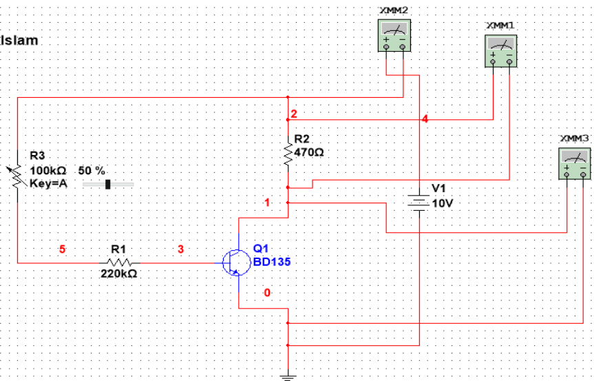
Fig : Fixed Bias Circuit (BD-135)
