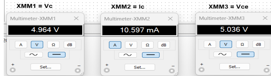
Fig : Fixed Bias Circuit (C828)
